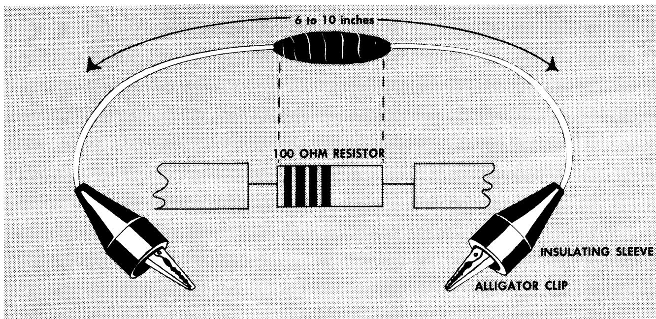
Fig. 5-13. Shorting strap useful in locating an unbalanced stage in a vertical or horizontal amplifier. Insulating tape covers the 100-ohm resistor.
