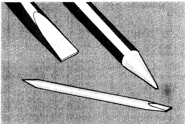
Fig. 5-10. A soldering aid constructed from a \frac{1}{4} -inch wooden dowel.
